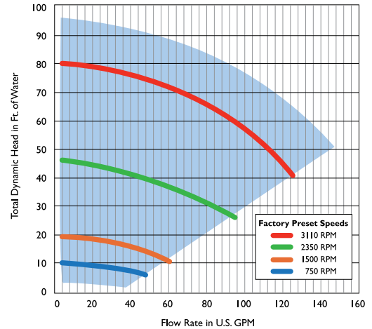
NOTE: The chart above demonstrates performance rates at factory preset speeds of 750 RPM, 1500 RPM, 2350 RPM and 3110 RPM. However, flow rates can also be custom programmed between the ranges of 400 RPM and 3450 RPM as indicated by the blue tint.
